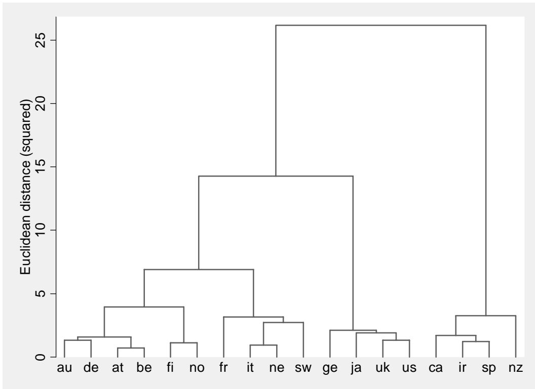
Figure 5. Cluster analysis
